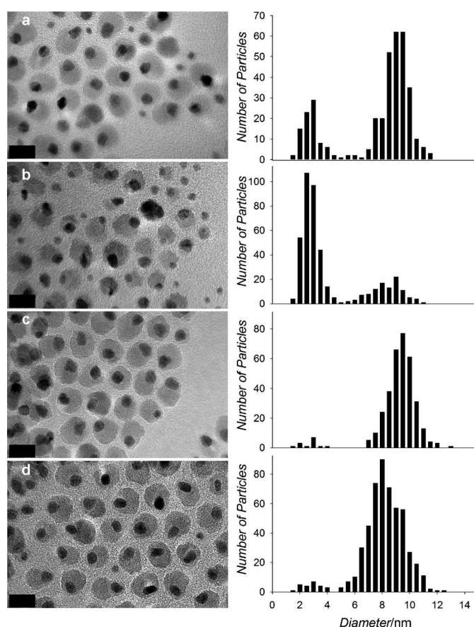
Figure 4. TEM images (scale bars are 10 nm) and size distribution histograms of a) the as-synthesized FePt-Fe 3 O 4 particles and the fractions from the DMCR peaks b) B', c) C', and d) D' in Figure 5.
