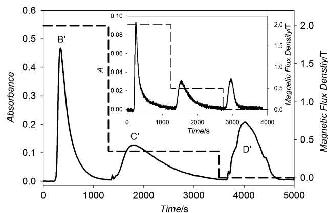
Figure 5. Chromatogram of preparatory-scale separation of FePt-Fe 3 O 4 (solid line) and the magnetic field program used (dashed line). Inset is analytical-scale separation of the same sample. Hexane mobile phase is used for all separations.
