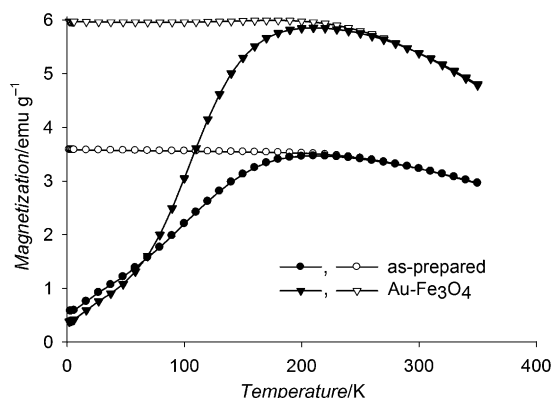
Figure 3. FC (open symbols) and ZFC (filled symbols) magnetization data. H = 100 Oe.
